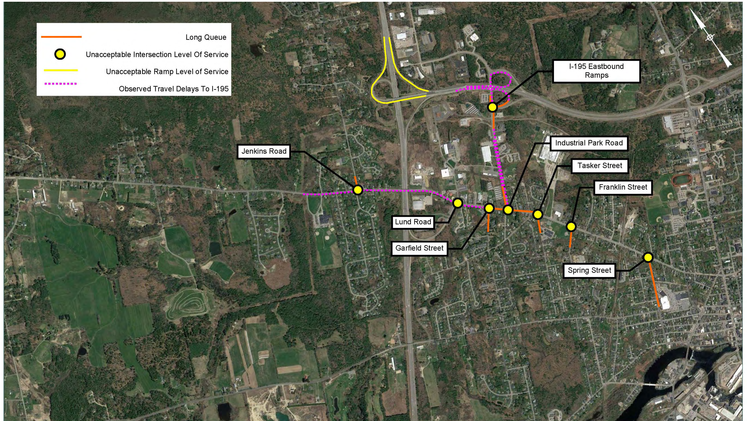
Saco Route 112/ Exit 36 Area Transportation Study Figure 2.14 - Existing Traffic Mobility Problem Locations
