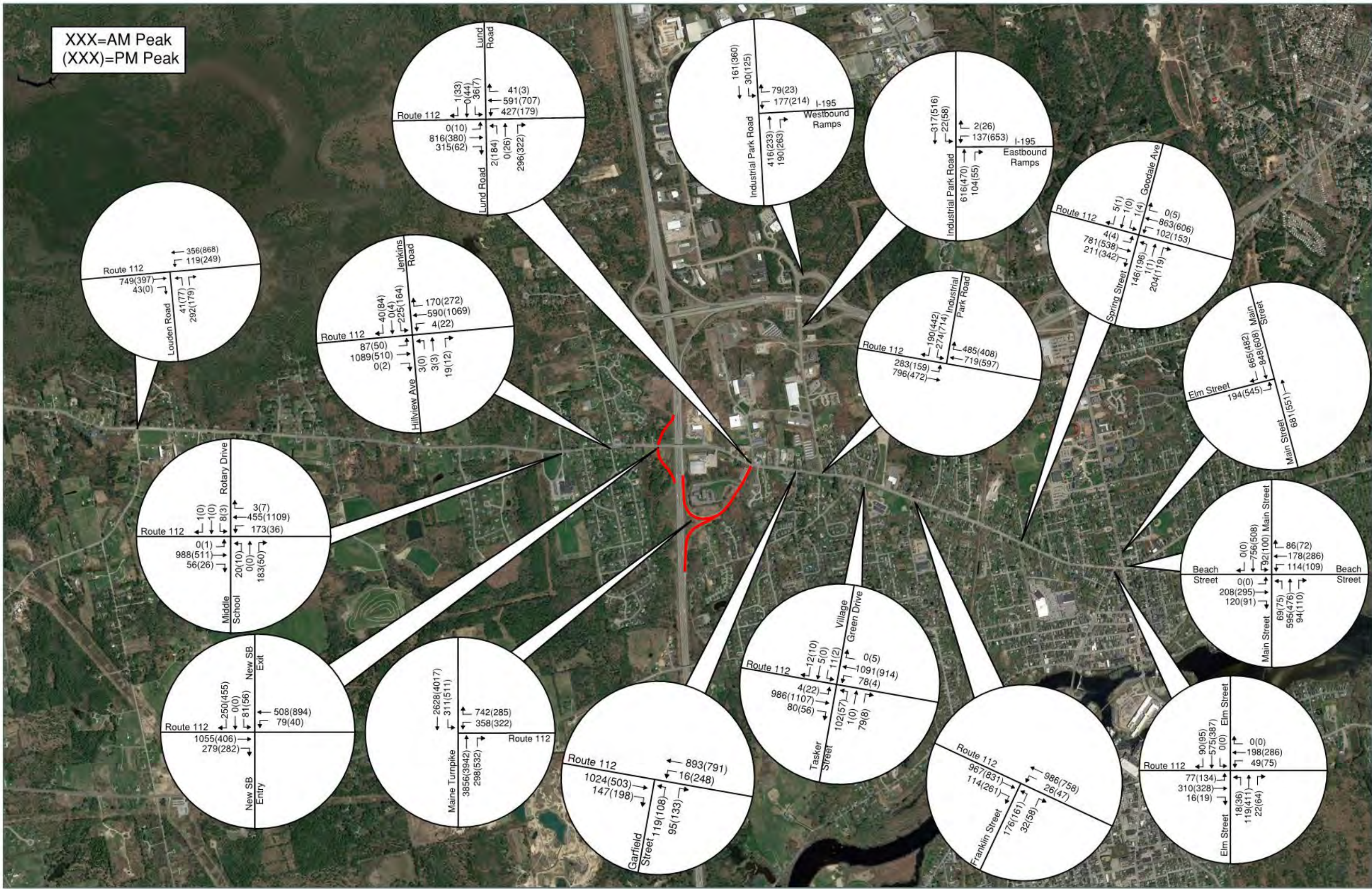
Figure 7.7 2040 Traffic Volumes Modification of Exit 36 (A4)
