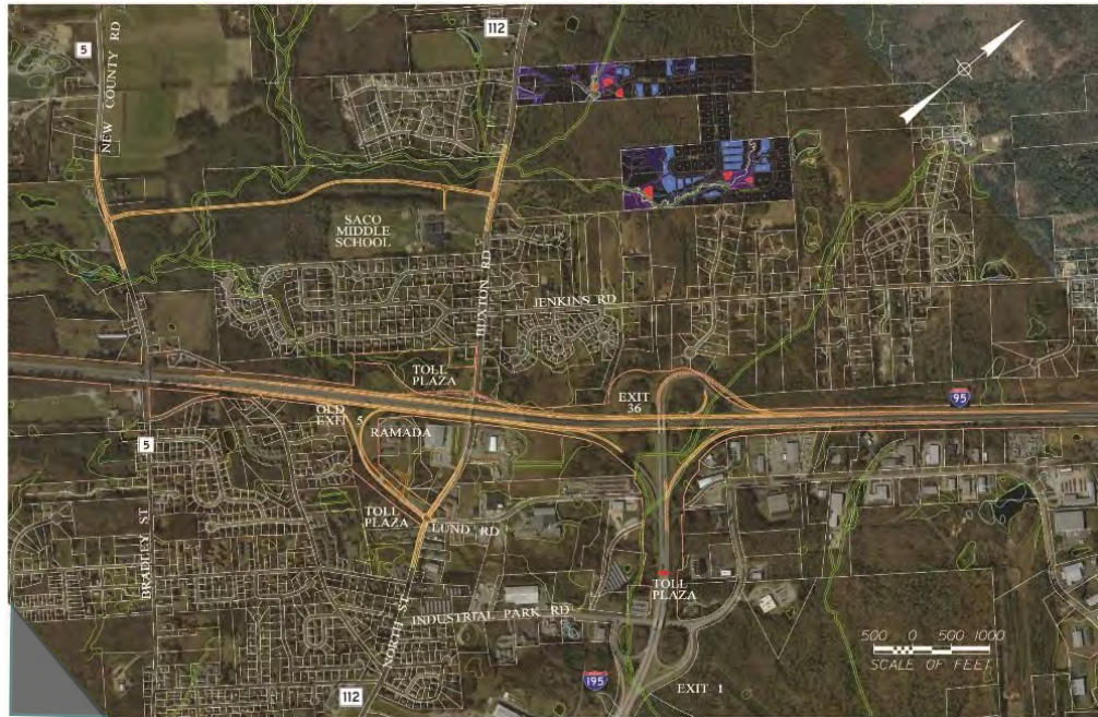
Figure ES.4: A6 - Modification of Exit 36 and Route 112 Route 5 Connector
