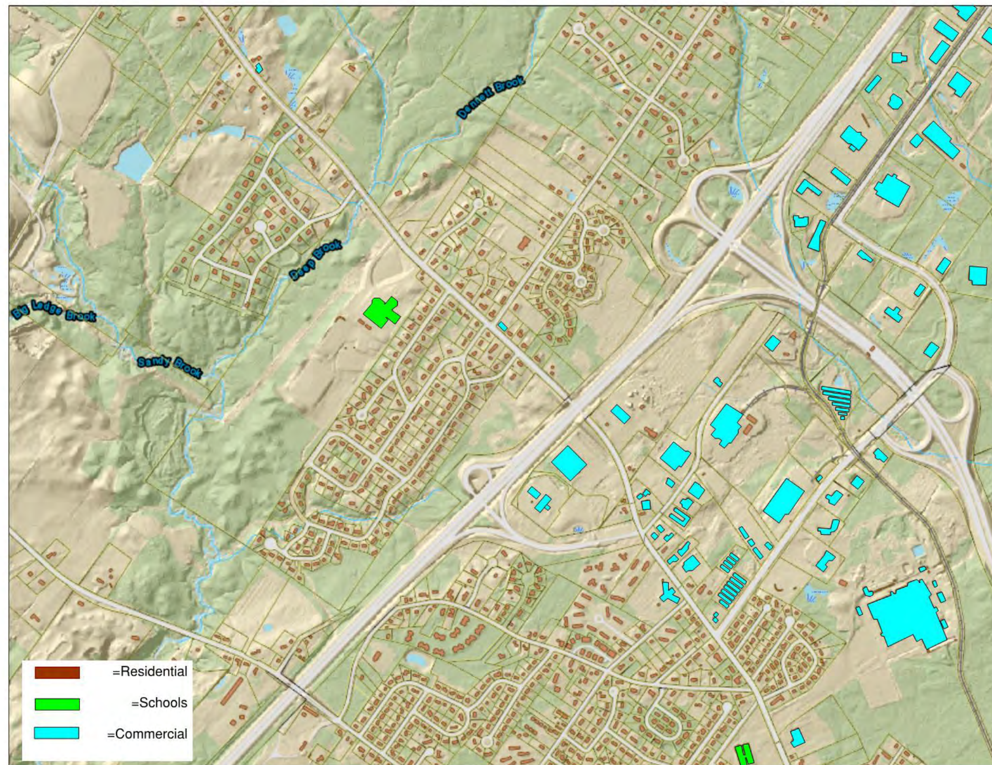
Route 112/ I-95 Exit 36 Transportation Study, Saco, Maine Figure 4.2: Lots and Building Plan Near Exit 36
