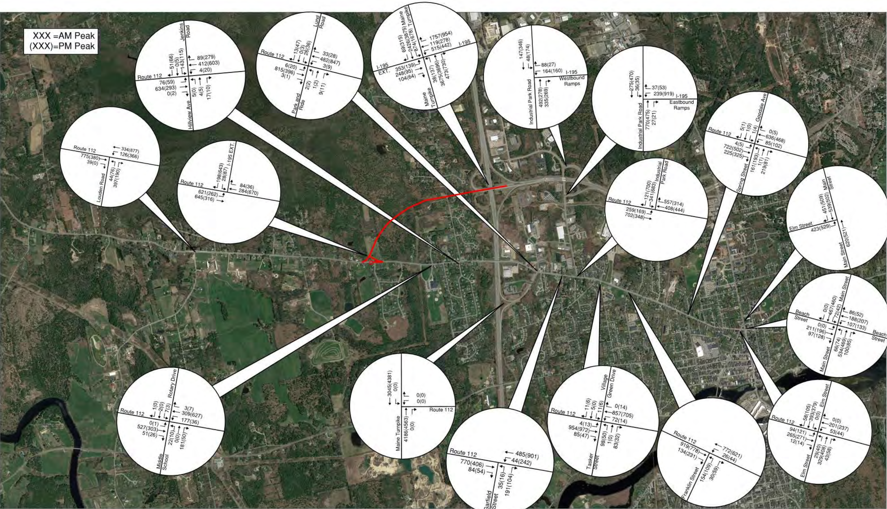
Figure 7.4 2040 Traffic Volume Extension of I-195 (A3)
