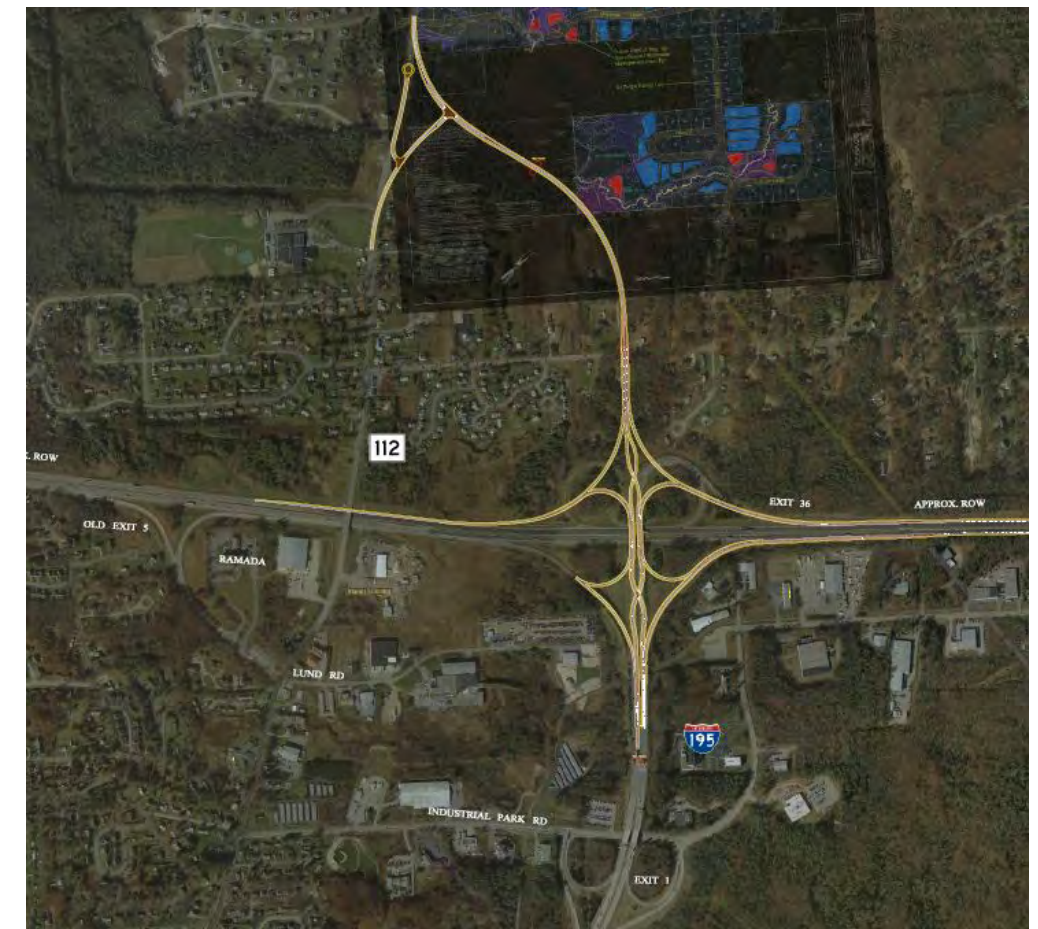
Figure 6.6 Diverging Diamond Signalized Interchange Configuration
