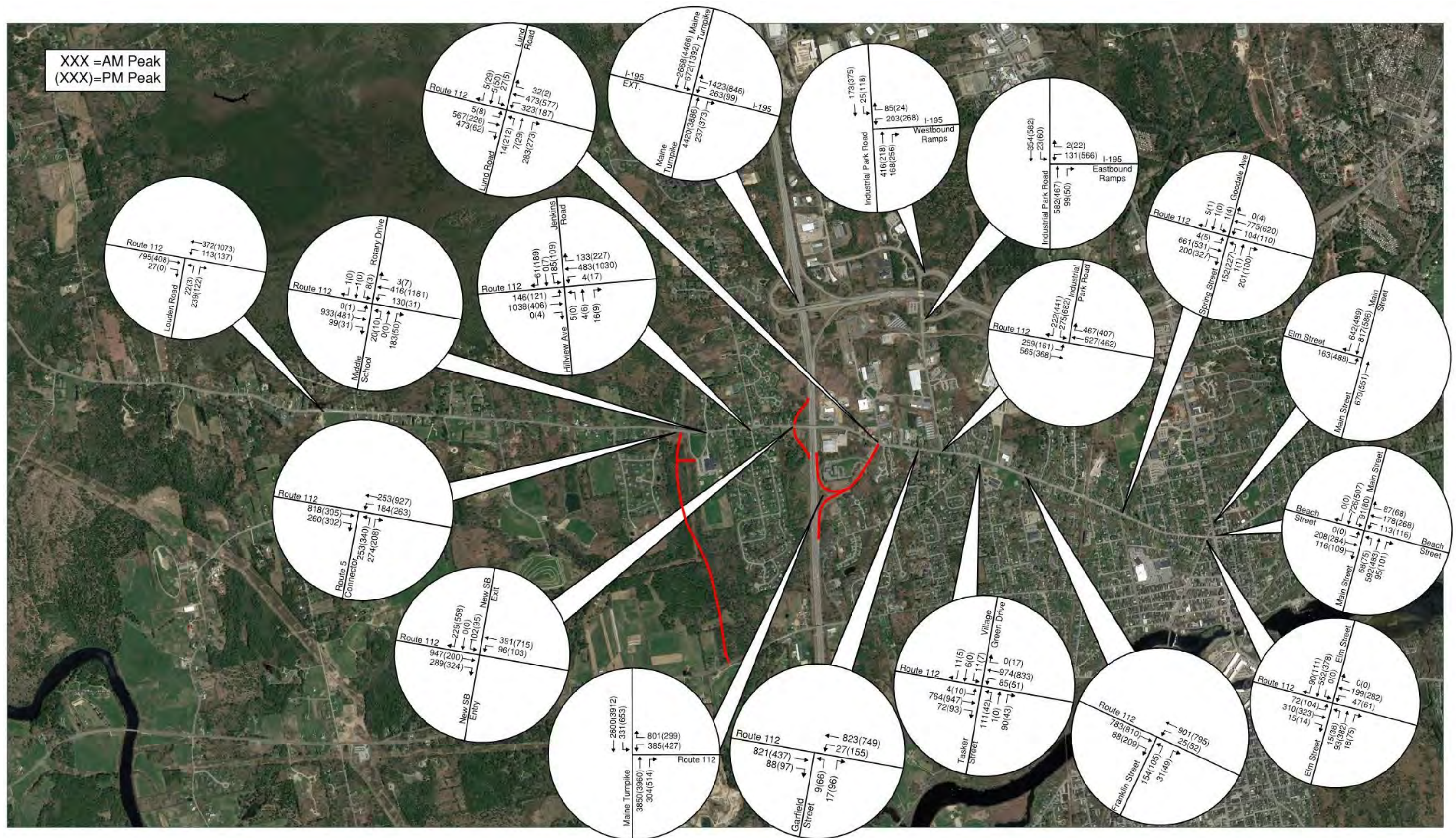
Figure 7.13 2040 Traffic Volumes Modification of Exit 36 and Route 112/Route 5 Connector (A6)
