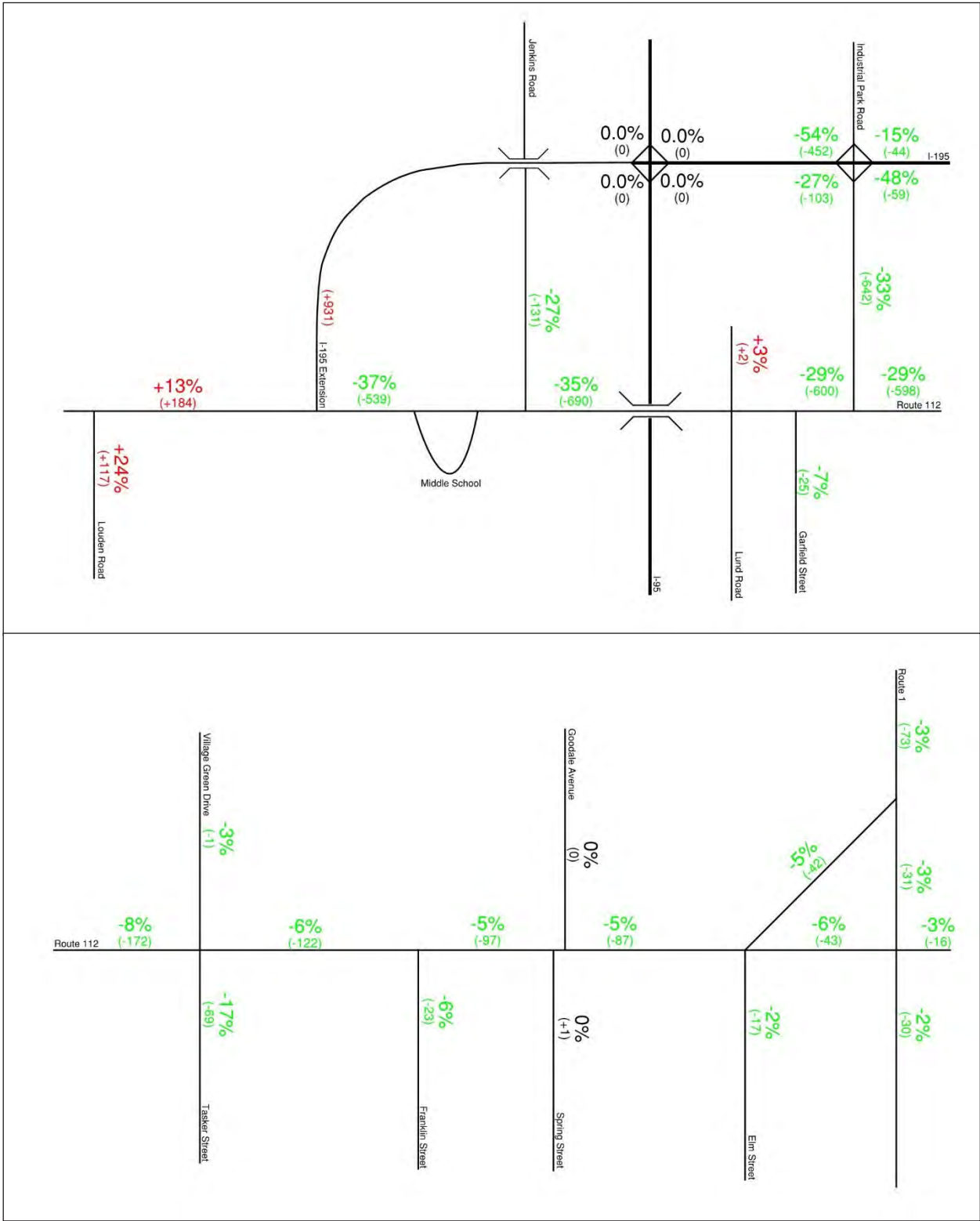
Figure 7.5 AM Peak Hour Comparison between A3 and 2040 No Build Volumes
