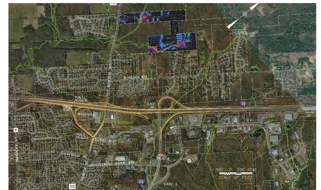
Figure ES.2: A4 - Modification of Exit 36
