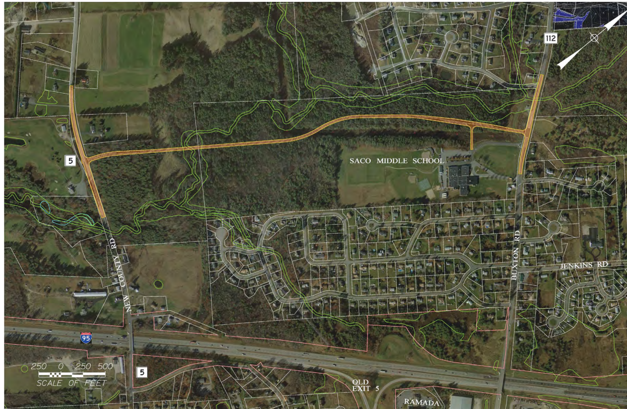
Figure 6.3: A5 - Route 112/Route 5 Connector Road
