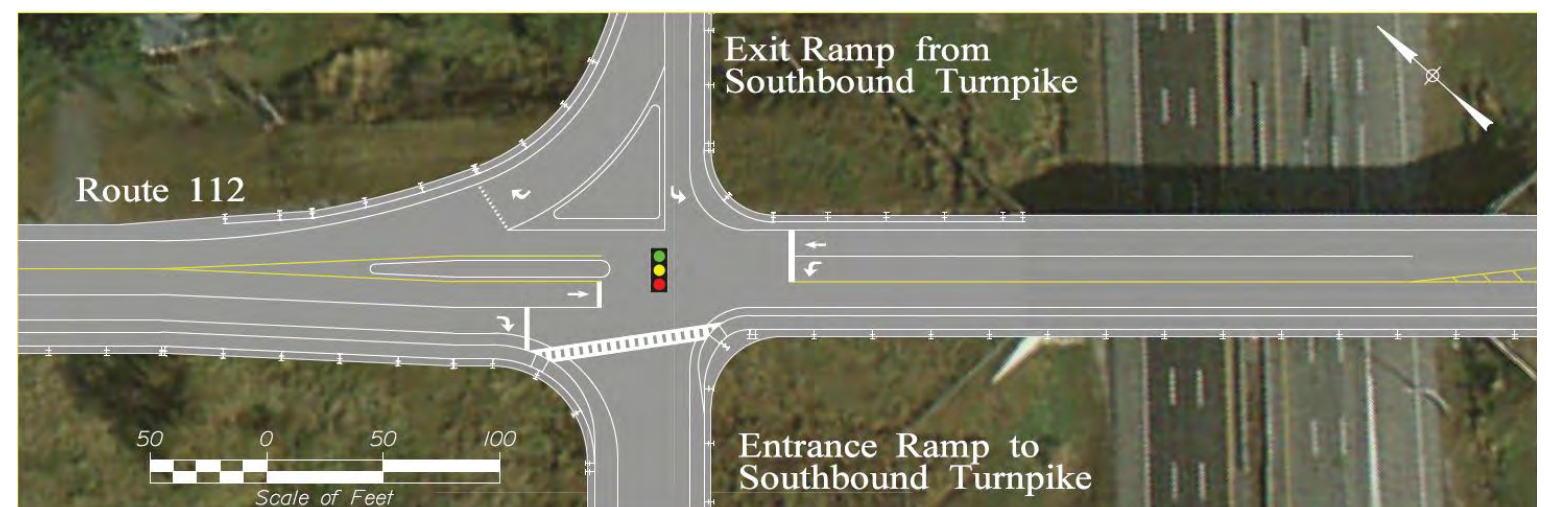
Figure 11.7 Exit 36 Route 112 Intersection
